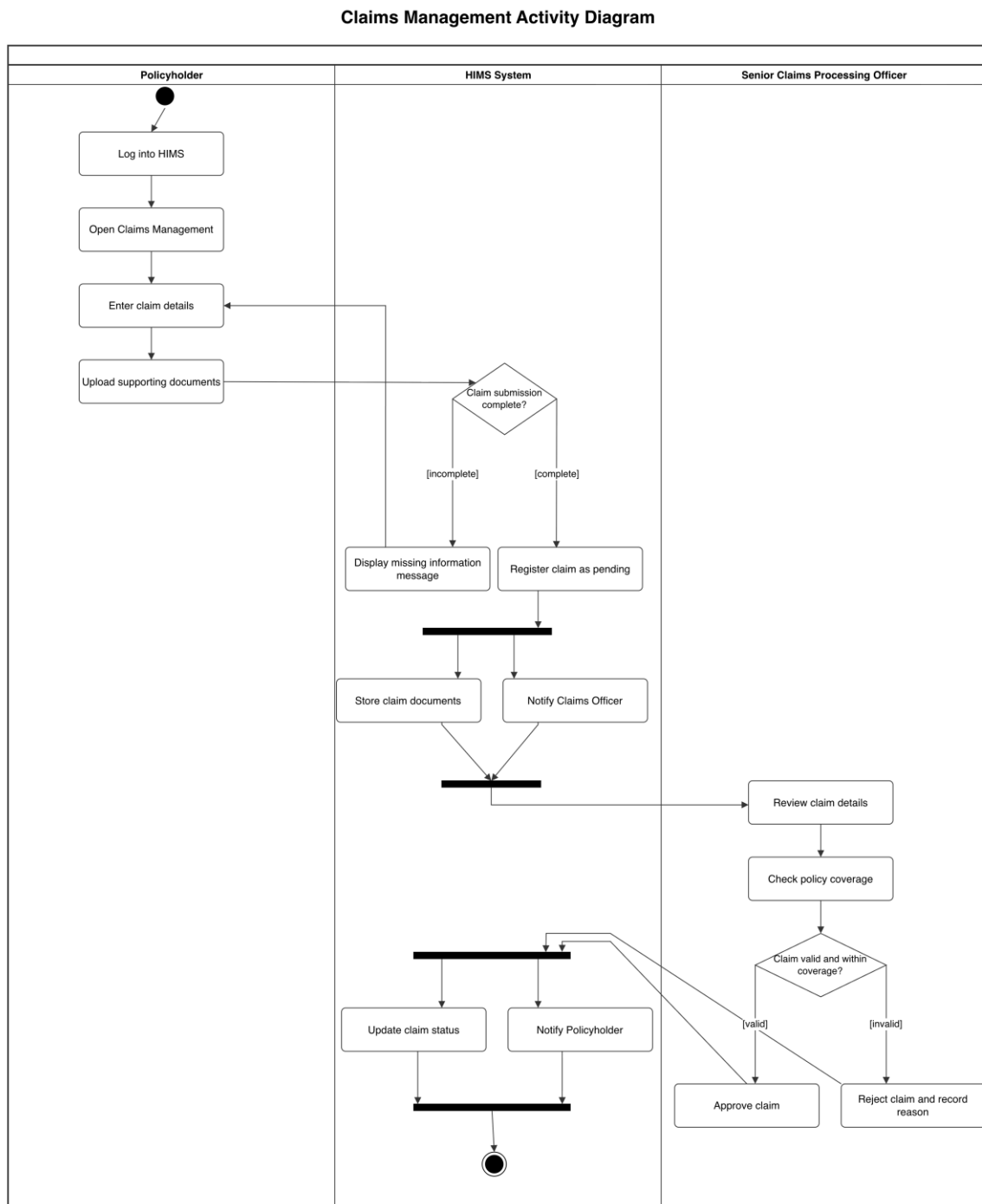
Figure 02: Claims Management Activity Diagram
