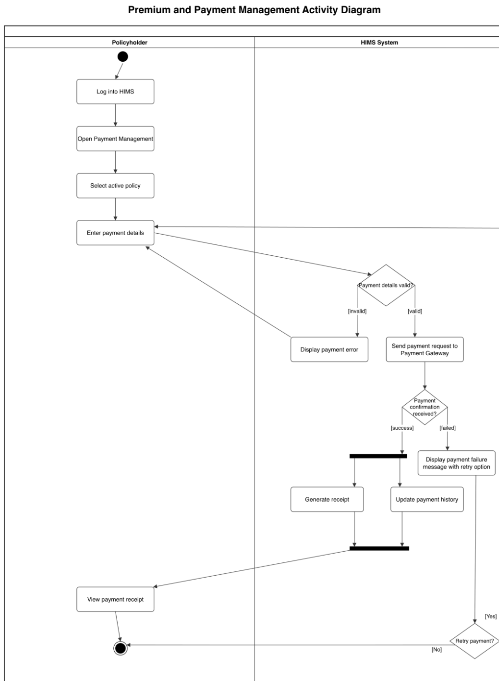
Figure 04: Premium & Payment Management Activity Diagram
