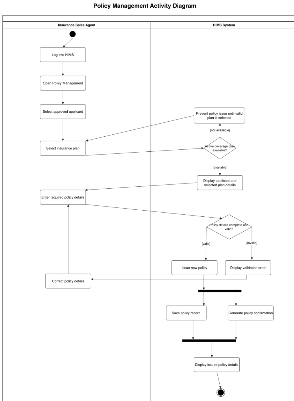
Figure 01: Policy Management Activity Diagram
