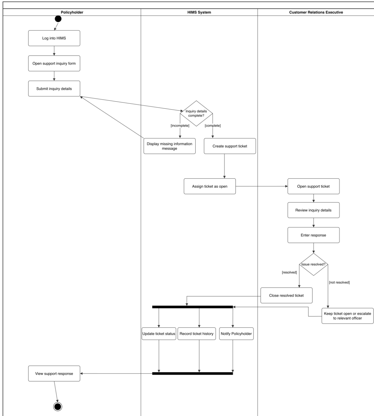
Customer Support and Inquiry Management Activity Diagram
